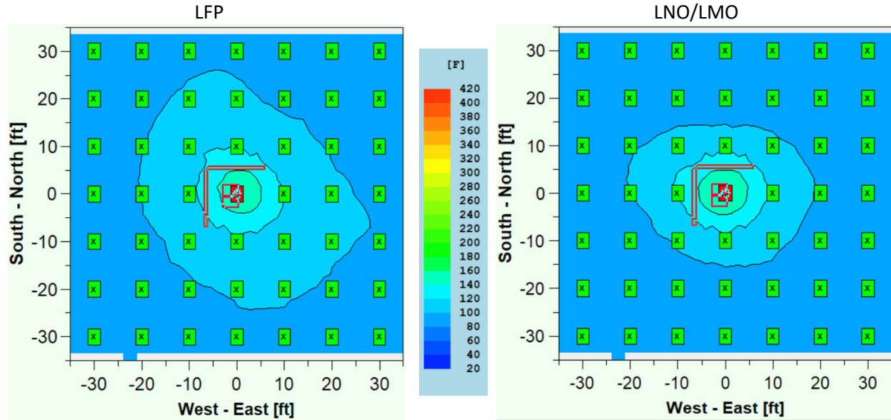
Figure 6-30: Contour plots of ceiling gas temperatures at first sprinkler operation during LFP (left) and LNO/LMO (right) tests. Convert to metric as [m = ft \times 0.305] and [^{\circ}C = (^{\circ}F - 32)/1.8] .
