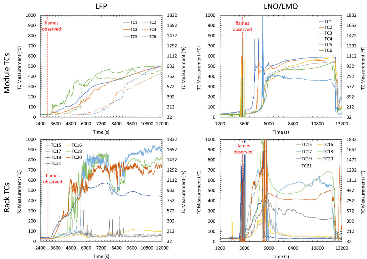
Figure 5-7: TC measurements during LFP (left) and LNO/LMO (right) tests for modules (top) and rack (bottom).
