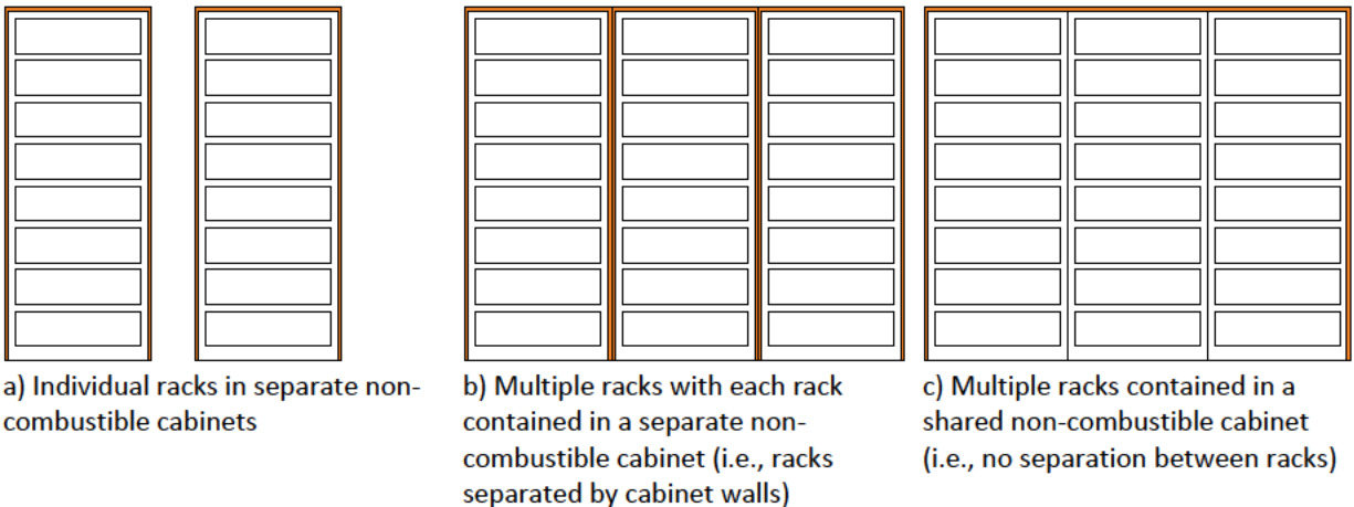
Figure 7-3: Elevation view of installation configurations for an ESS comprised of multiple racks.
