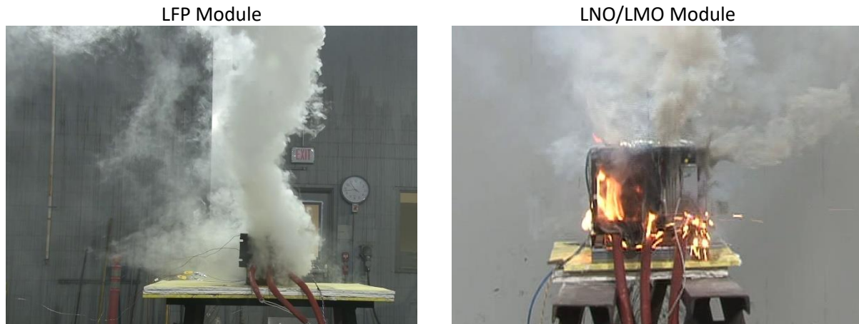
Figure 4-6: Example of LFP (left) and LNO/LMO (right) battery response to abuse conditions. LFP batteries vented a thick white smoke and sometime required an external pilot flame to ignite, whereas LNO/LMO batteries generate sparks that consistently ignited vent gases.
