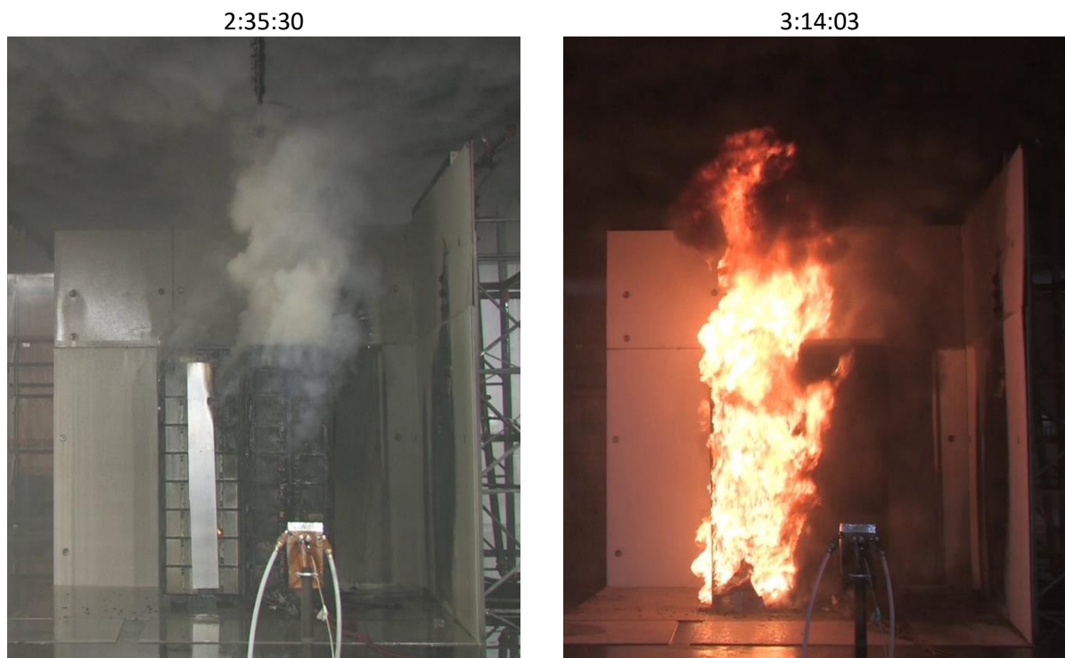
Figure 6-23: Photos of LNO/LMO sprinklered test during fire development on target rack: view of rack once sprinklers were shut off (left) and fire size when sprinklers were turned back on (right).
