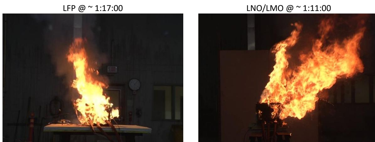
Figure 4-8: Photos of LFP (left) and LNO/LMO (right) at near peak heat release rate. The angle of the flames is due to the momentum of the vent gases exiting the batteries.
