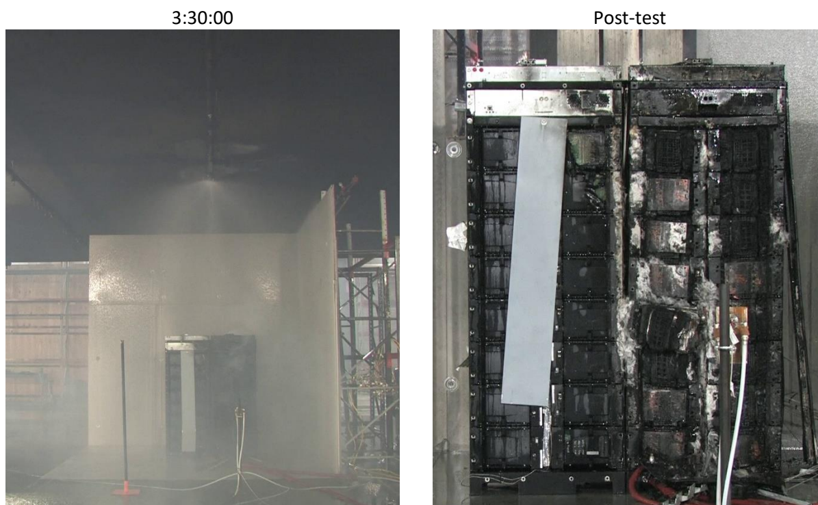
Figure 6-21: Photos of LFP sprinklered test during fire decay phase (left) and at burnout (right).
