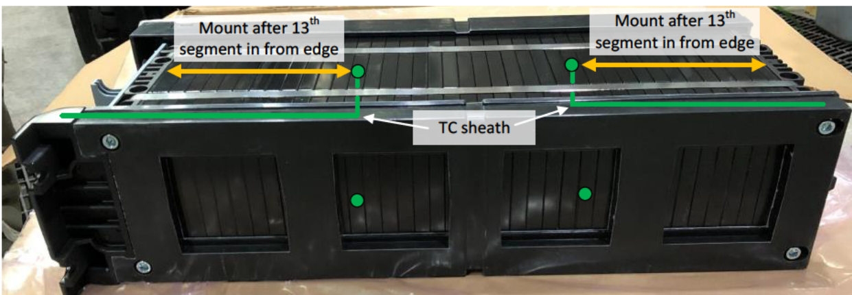
Figure 4-2: Thermocouple layout, LFP
