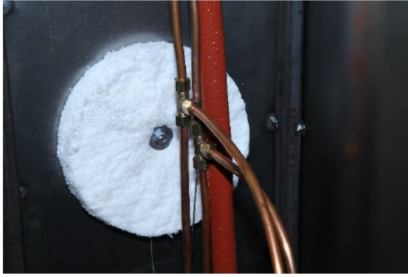
Figure 3-8: Photo of backside of TCs installed on mock ESS rack (TC28 – 37) on left and schematic of TC attachment on right.
